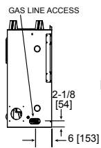
SL-550TR & TRS Side View
